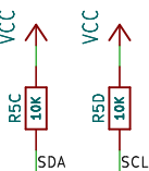
I2C Pullups
