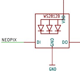
NEOPIXEL
