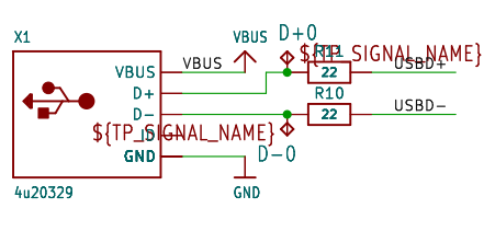
MICRO USB
