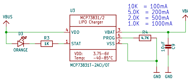
LIPO CHARGING
