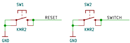
RESET/USER SWITCHES
