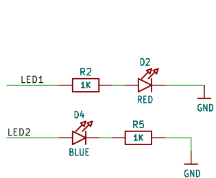
INDICATOR LEDS
