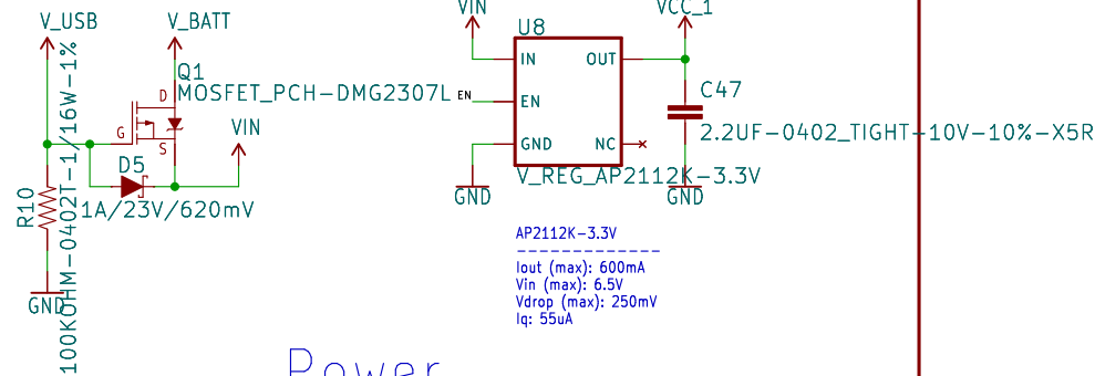
Power
