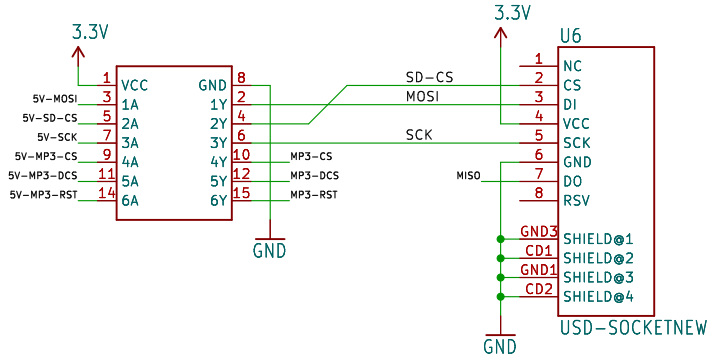
microSD
