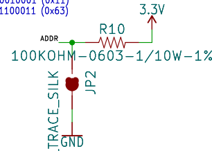
Address Select Jumper
