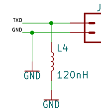
RxTx Antenna Connector
