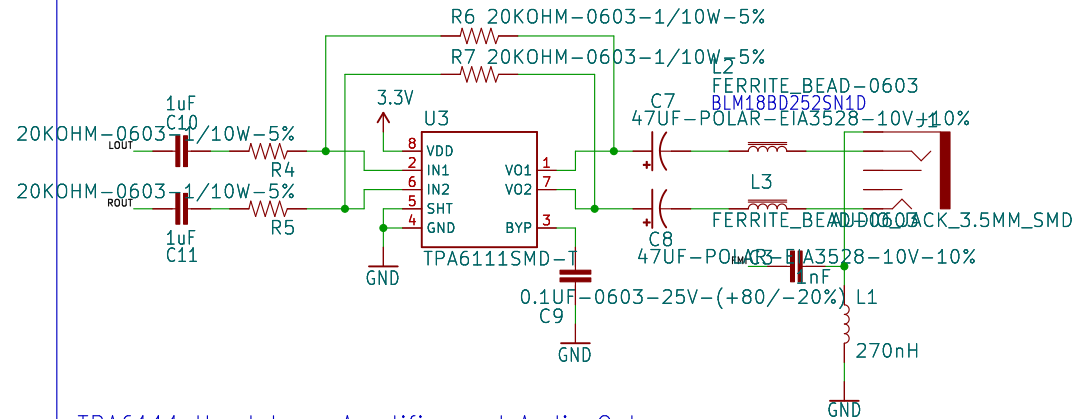
TPA6111 Headphone Amplifier and Audio Out
