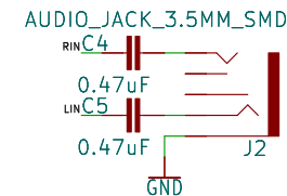
Line Level Audio Input Jack
