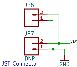
Battery Connector 2.0-6.0V
