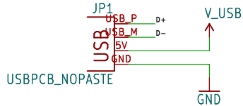
USB Plug
