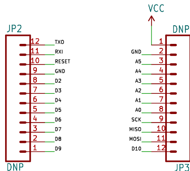
GPIO Headers
