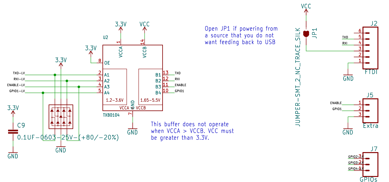
Interface and Logic Conversion
