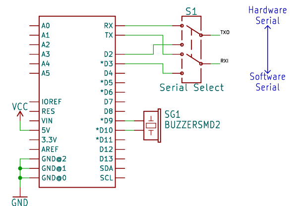
Shield and Serial Select
