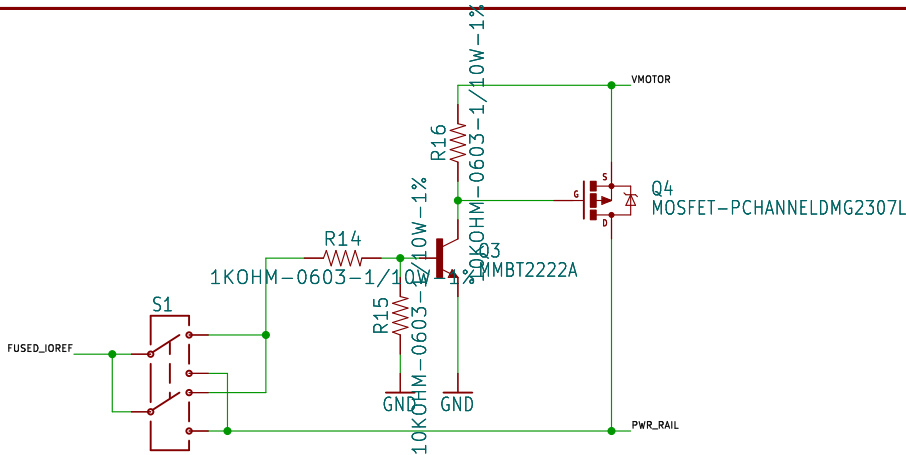
Power Rail Select Switch
