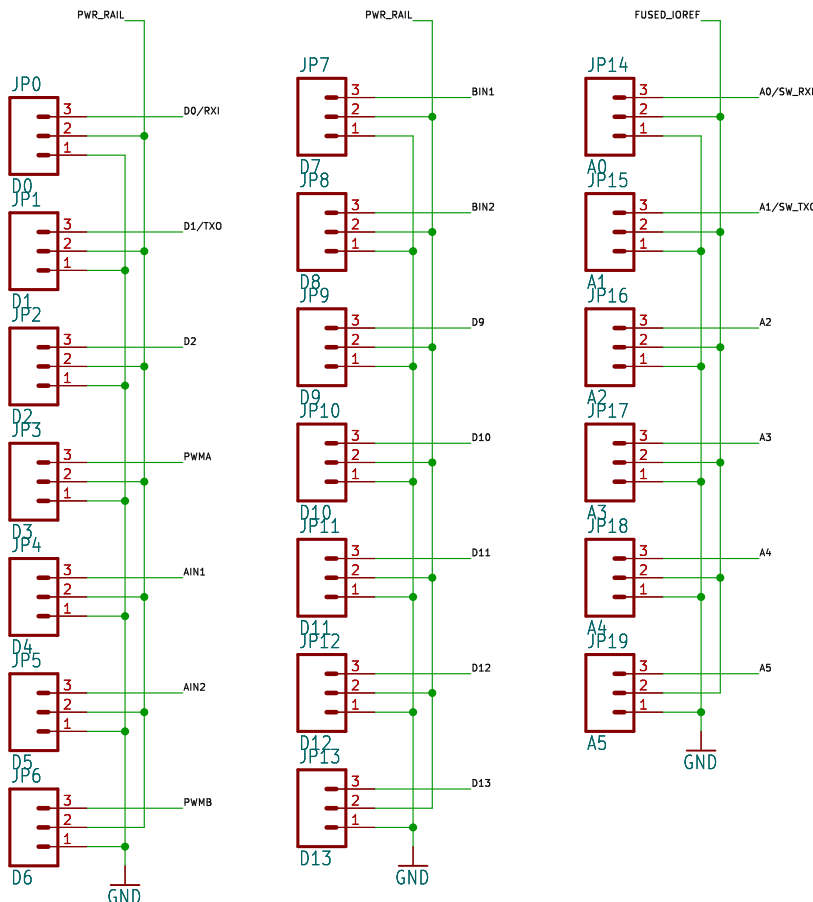
3 Pin Header Field
