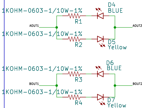
Motor Outputs
