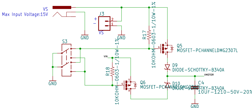
Power Input Select Switch
