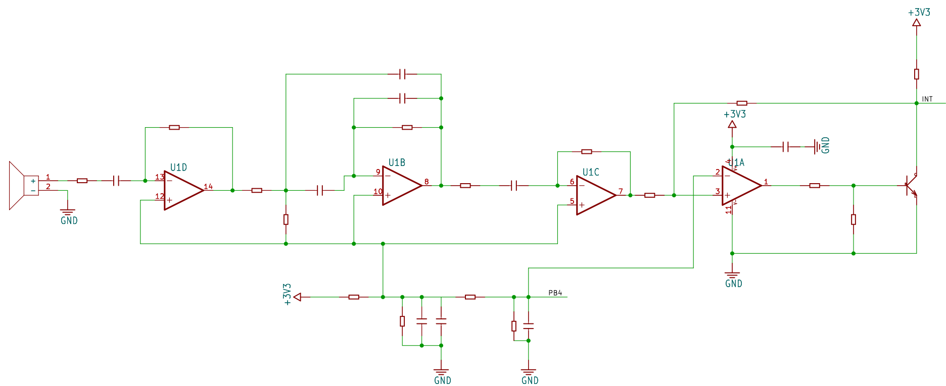
Ultrasound reception STM8
