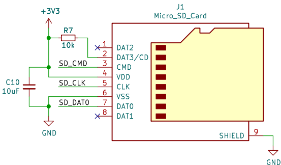
Micro-SD card
