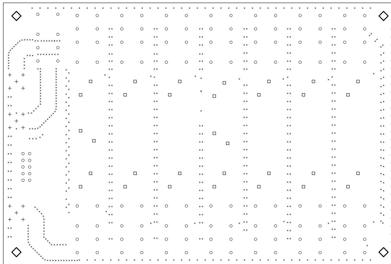
Drill Map:
