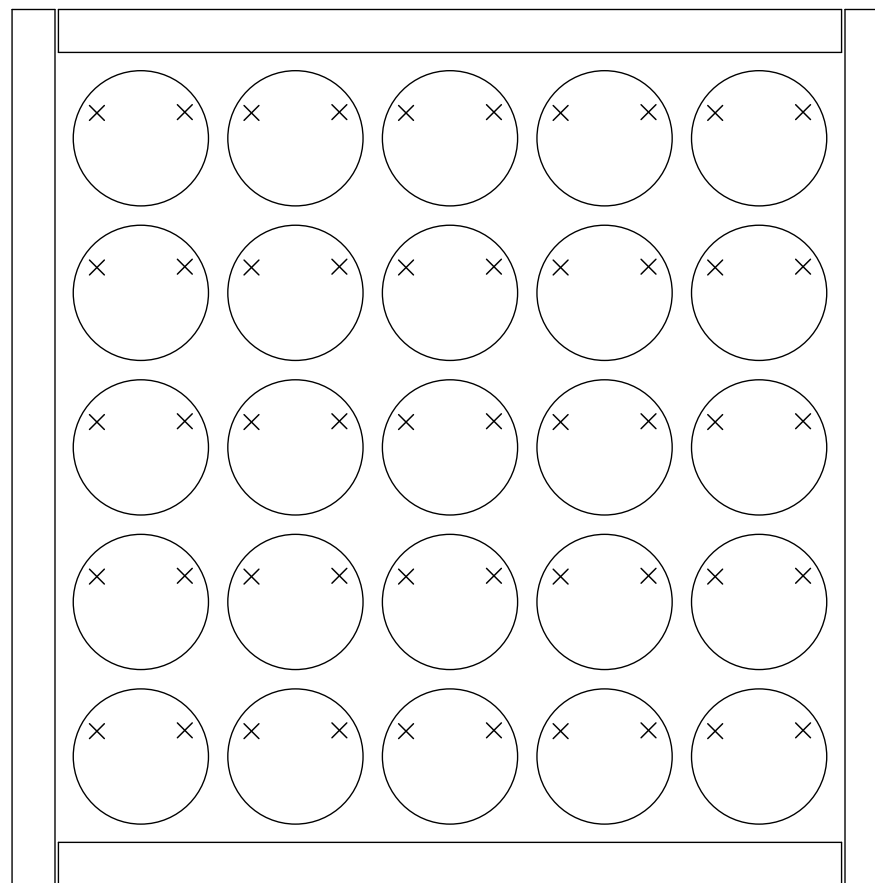
Drill Map: × 2.200mm / 0.0866" (50 holes)
