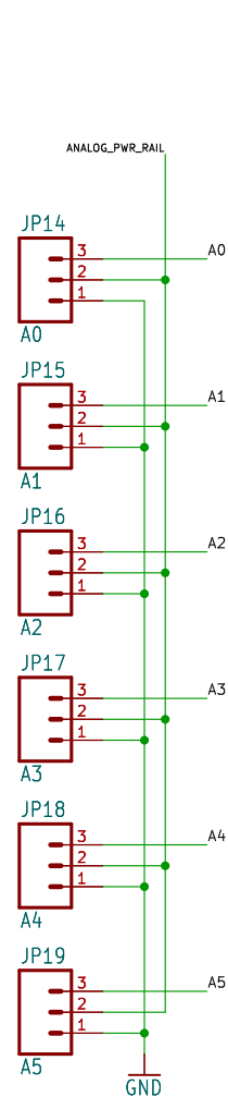
Analog 3 Pin Headers
