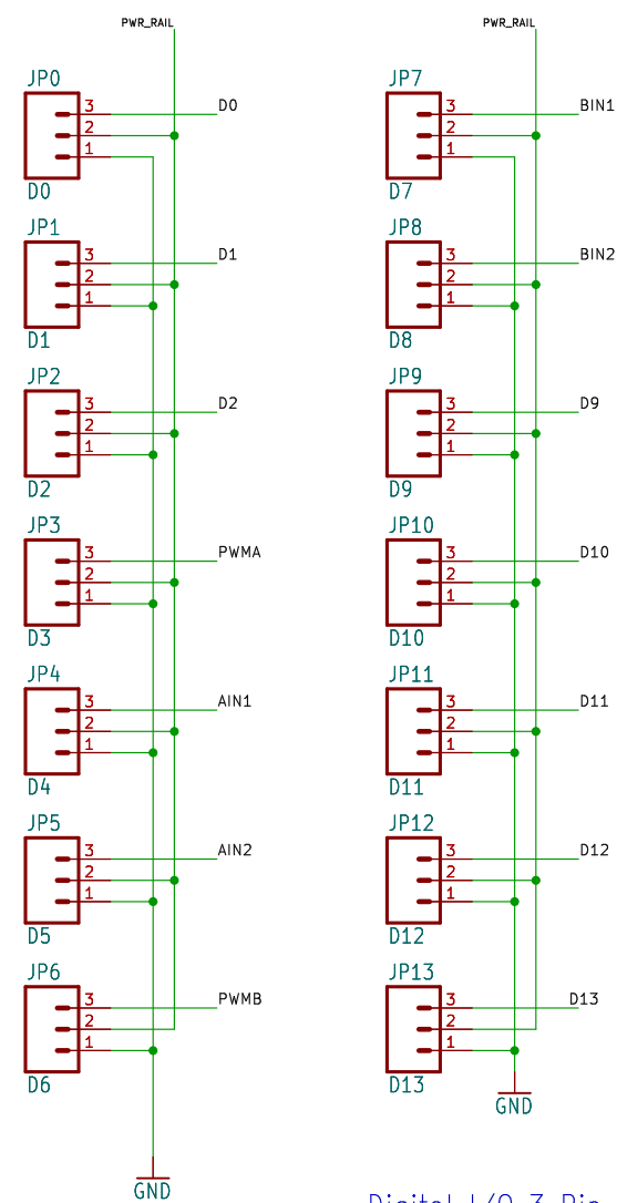
Digital I/O 3 Pin Headers
