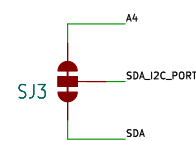
Jumpers to select between SCL / A5 and SDA / A4 pins on the new R3 footprint – for Leonardo compatibility.
