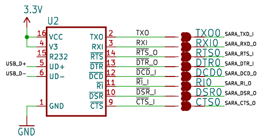
USB to Serial
