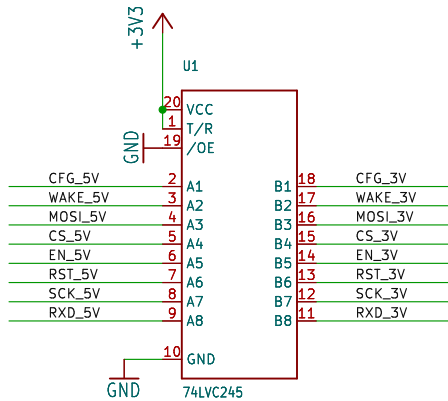
Level Shifter
