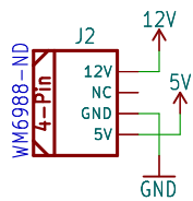
COMPUTER-PERIPHERAL-POWER
