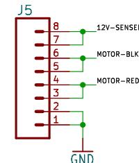
Motor Controller Output
