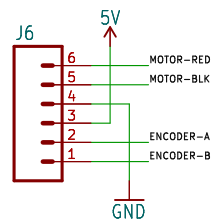
Motor Connect
