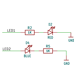
INDICATOR LEDS
