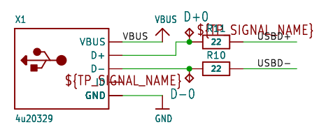
MICRO USB
