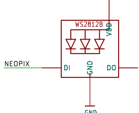
NEOPIXEL
