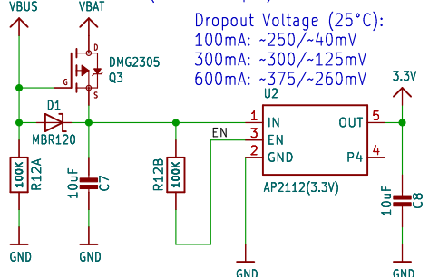
POWER AND FILTERING (600mA Output)
