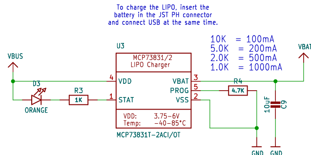
LIPO CHARGING
