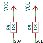
I2C Pullups
