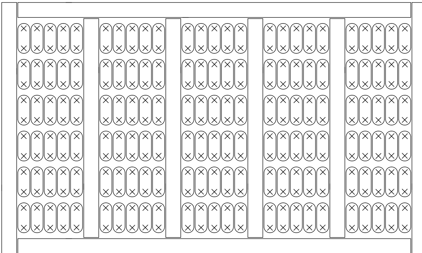
Drill Map: X 2.200mm / 0.0866" (300 holes)
