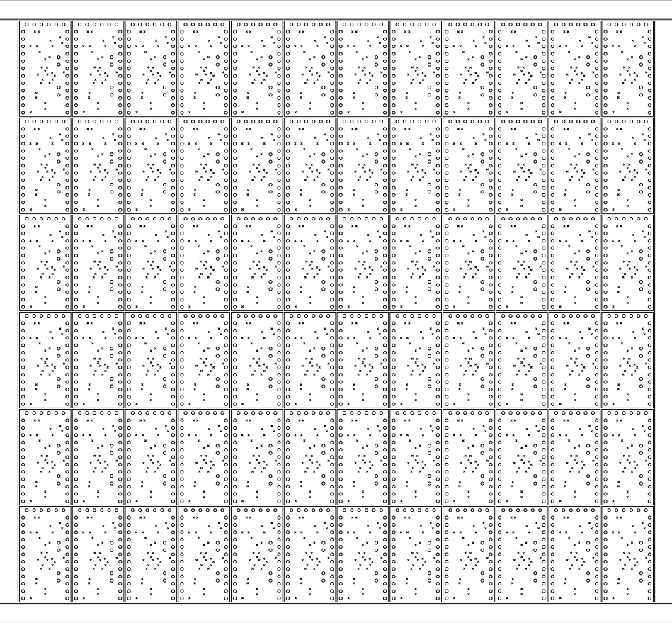
Drill Map: • 0.508mm / 0.0200" (2016 holes) ◦ 1.016mm / 0.0400" (2448 holes)
