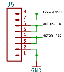
Motor Controller Output
