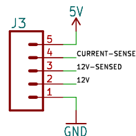
Current Sense
