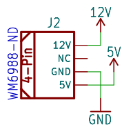
COMPUTER-PERIPHERAL-POWERRA Motor Connect
