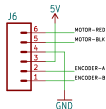
COMPUTER-PERIPHERAL-POWERRA Motor Connect
