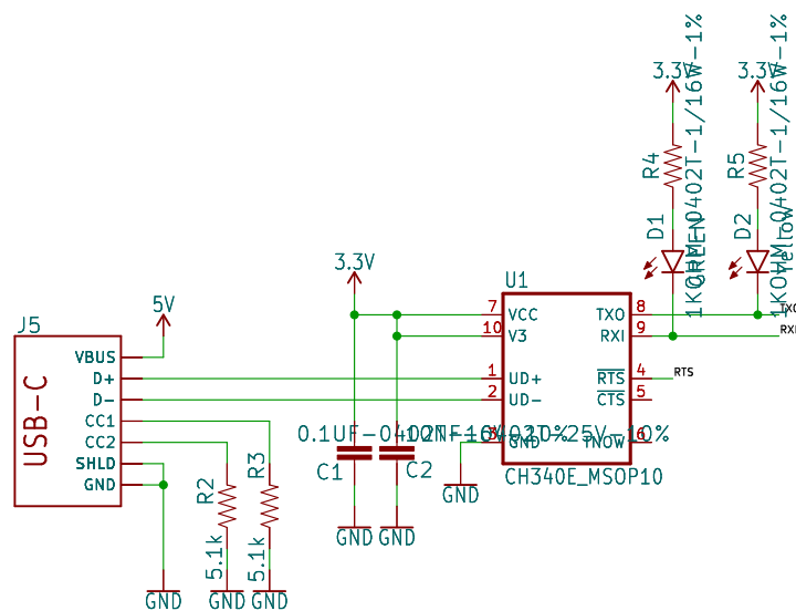
USB-to-Serial Converter
