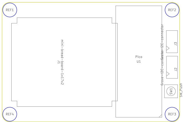
Copper Keepouts shown on Dwgs layer
