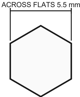
END VIEW
