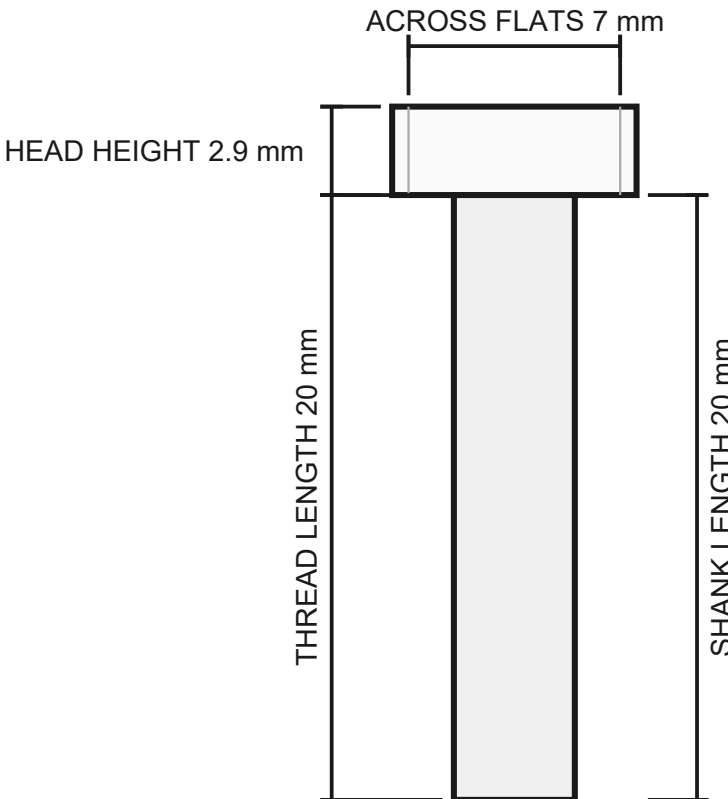
SIDE VIEW
