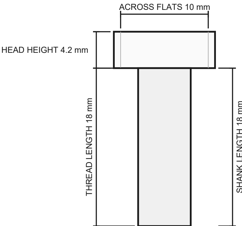
SIDE VIEW
