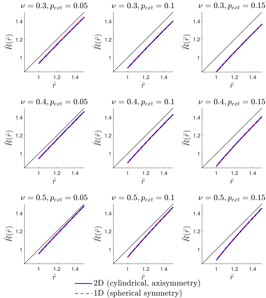
Figure 1.1 Results of the benchmark test for various Poisson ratio and external pressure values.
