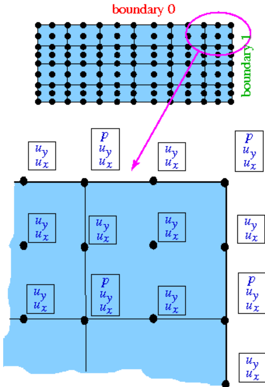
The sketch illustrates the degrees of freedom at each node before any FaceElements are attached.
