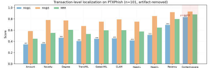
Fig. 7. Transaction-level localization on PTXPhish ( n=101 , artifact-removed). Our content-aware fusion is SOTA, beating every heuristic, MIL baseline, and the recency prior at Hit@1 ( p=0.002 ).
