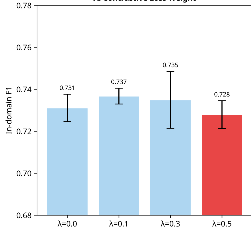
A. Contrastive Loss Weight
