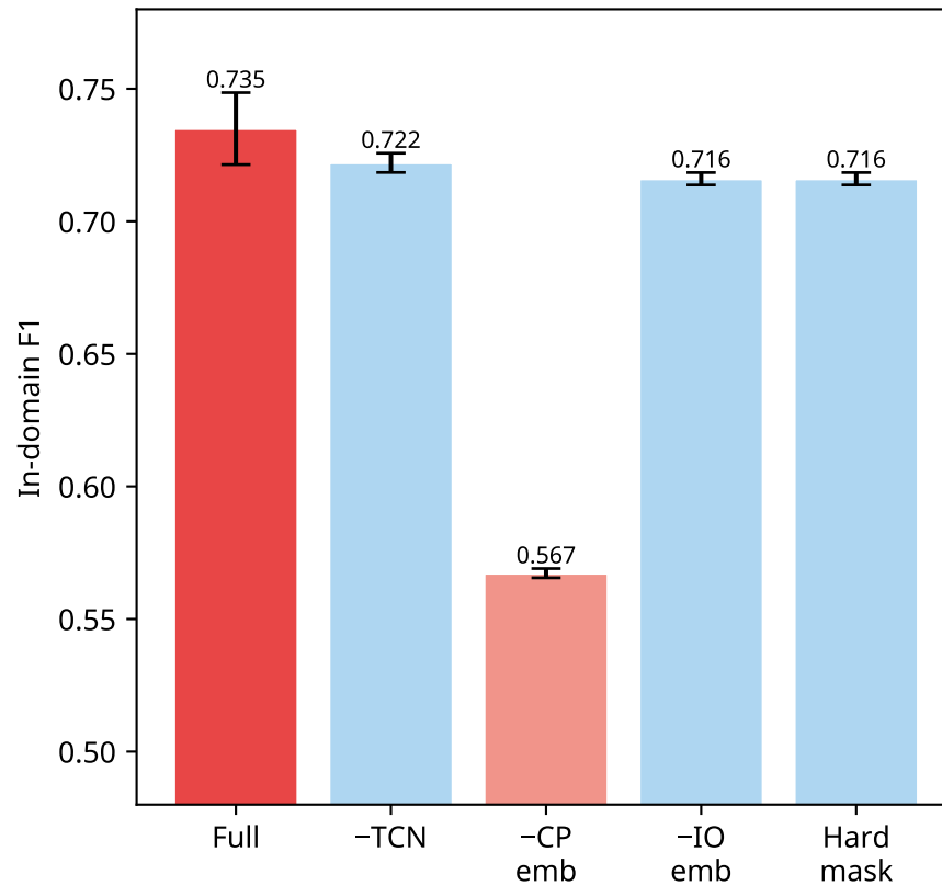
B. Backbone Components
