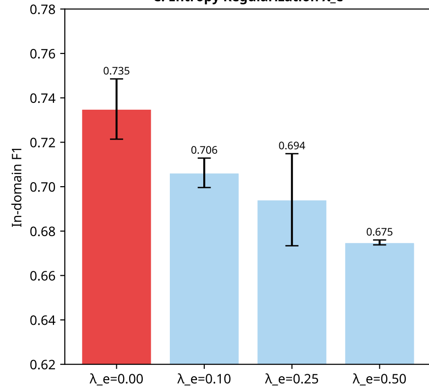
C. Entropy Regularization \lambda_e
