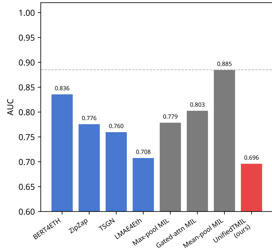
Hard-negative X-AUC hard
