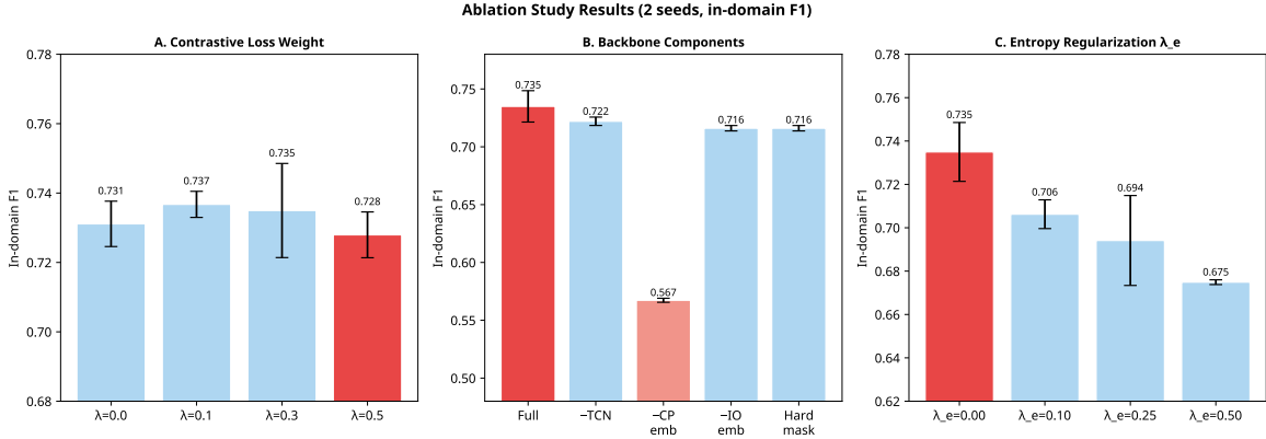
Fig. 4. Ablation Study Results (2 seeds, in-domain F1). (A) Contrastive loss weight. (B) Backbone components. (C) Entropy regularization. Removing CP embeddings causes the largest performance drop ( -23\% ).
