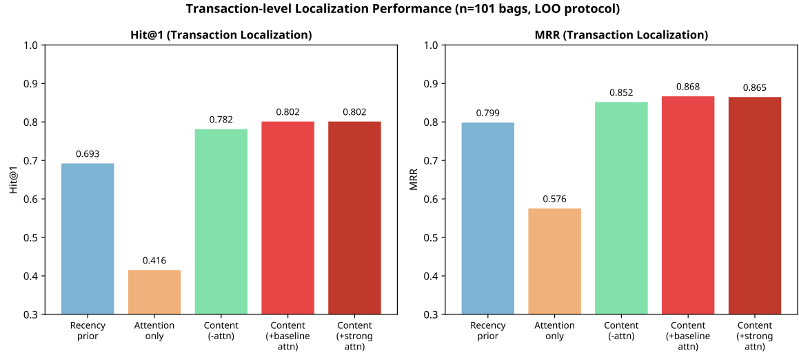
Fig. 3. Transaction-level localization performance. UnifiedTMIL (Streamlined) achieves strong localization without positional bias.
