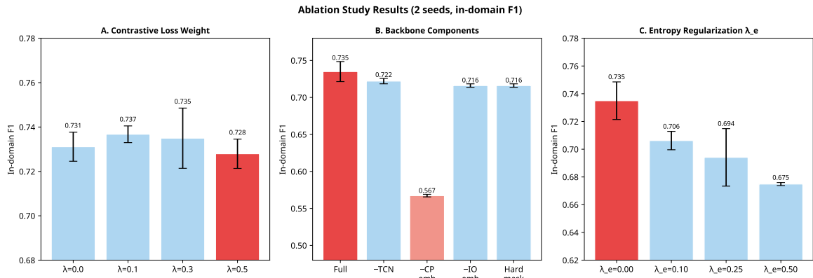
Fig. 4. Ablation Study Results. The combination of contrastive loss and backbone components provides significant lift over baseline configurations.
