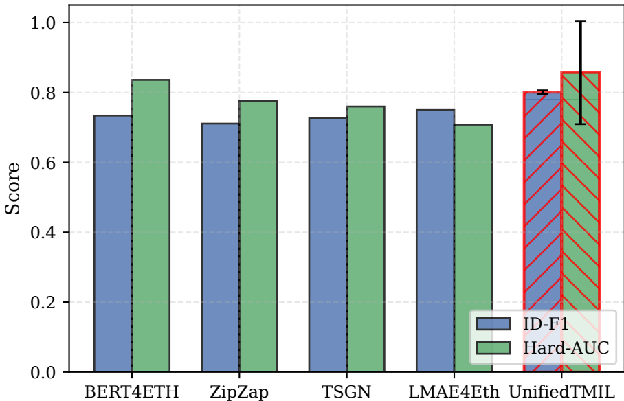
Account-Level Phishing Detection Performance
