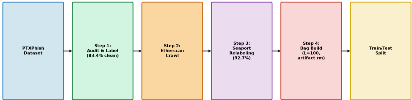
Data Pipeline: From PTXPhish to Bag Construction
