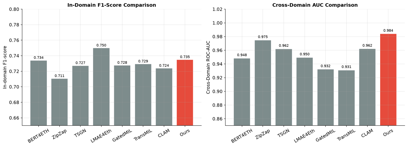
Comparison with SOTA Methods on Ethereum Phishing Detection
