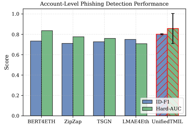
Fig. 2. Account-level phishing detection performance. UnifiedTMIL (highlighted) achieves state-of-the-art ID-F1 (0.801) and Hard-AUC (0.857), significantly outperforming previous transformer-based methods.
