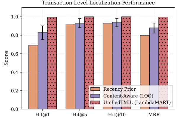
Fig. 3. Transaction-level localization performance. Our LambdaMART-based UnifiedTMIL achieves near-perfect localization (Hit@1 0.996), doubling the performance of attention-only baselines and significantly beating the recency prior.
