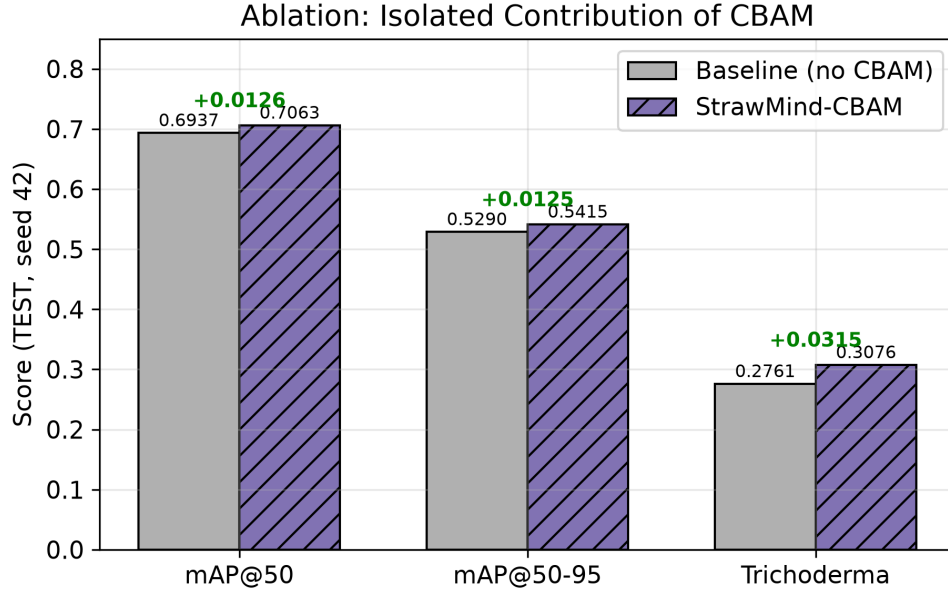
Figure 6: Isolated effect of CBAM (seed 42). CBAM provides +0.0126 overall mAP@50 and +0.0315 on Trichoderma , confirming attention—not augmentation—drives the gain.
