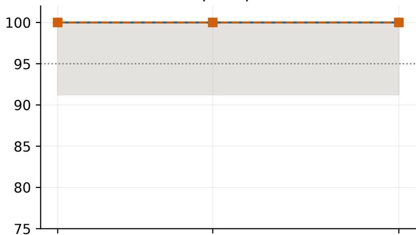
8 prompts
