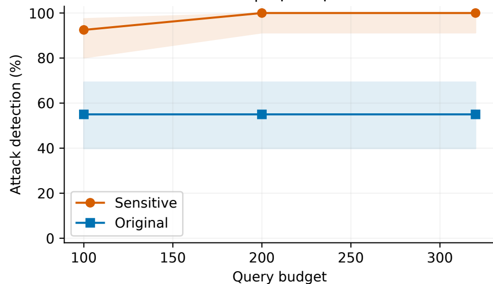
Top sensitivity | 4 prompts
