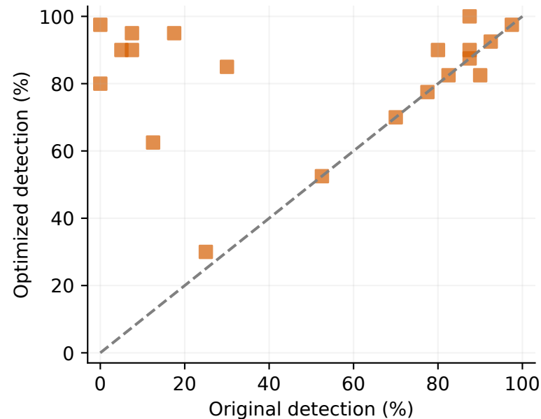
JS optimized
