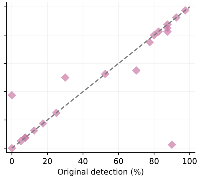
Logit optimized
