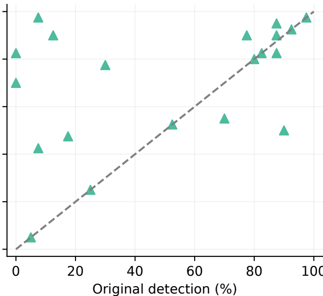
Top-K optimized
