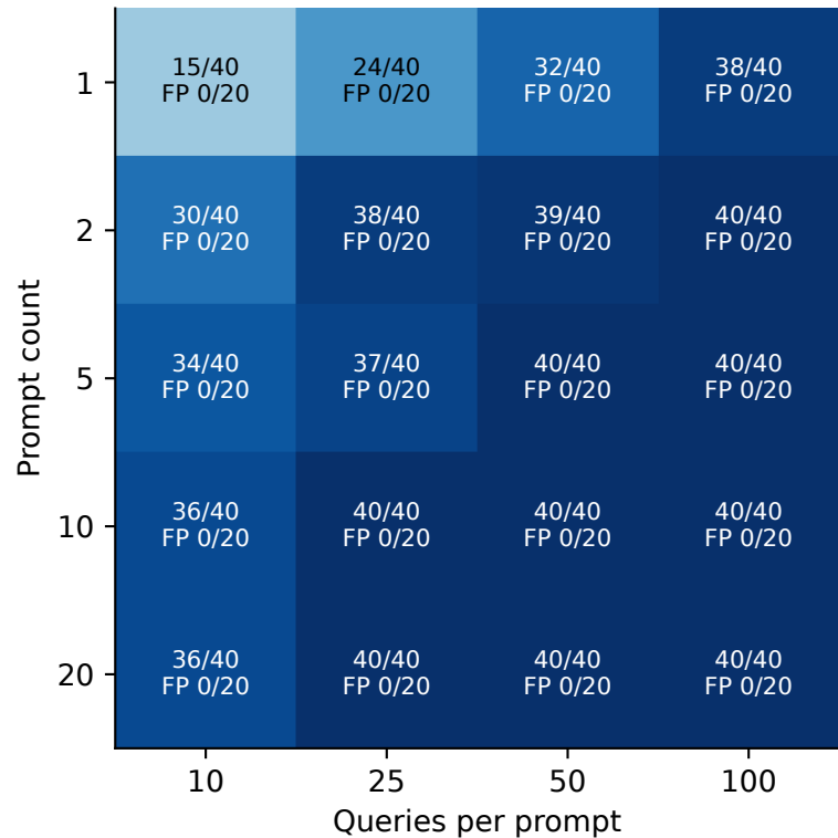
Sensitive ranked
