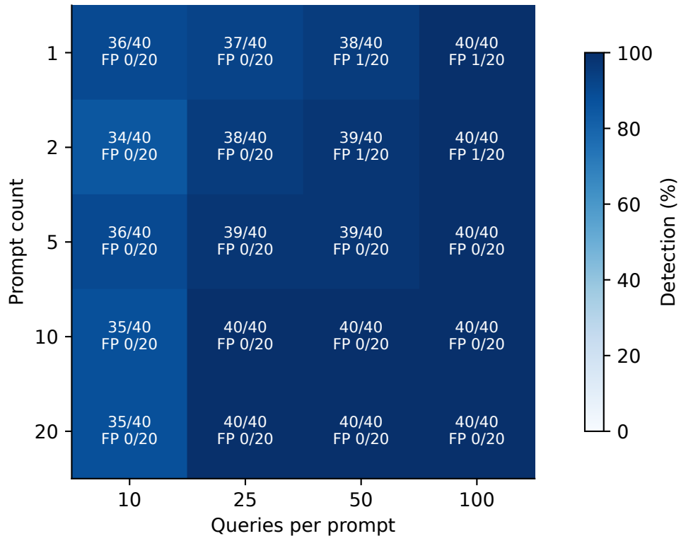
Ordinary ranked
