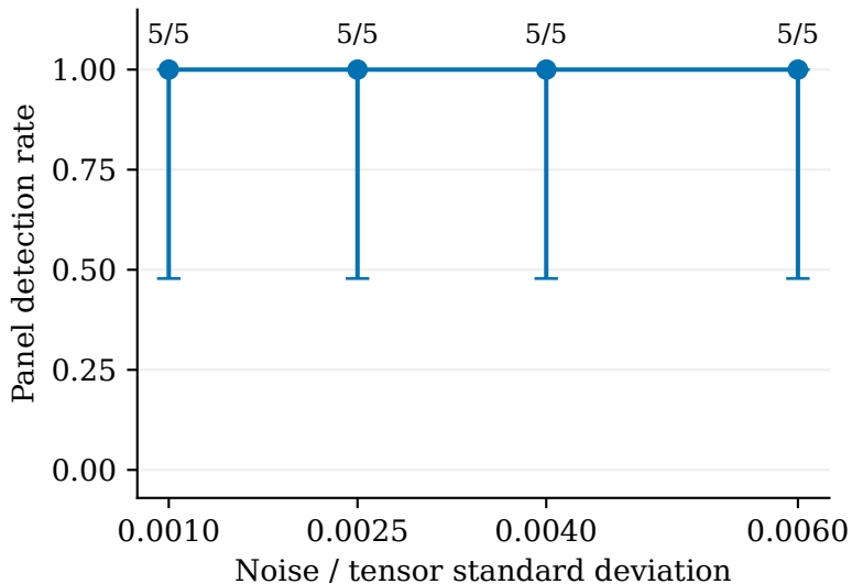
Gaussian perturbations
