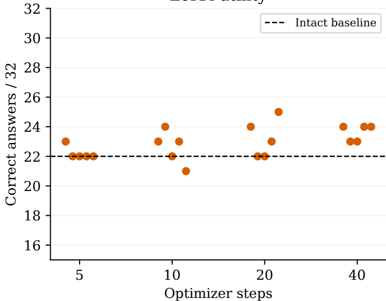
LoRA utility
