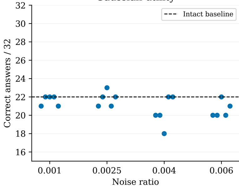
Gaussian utility
