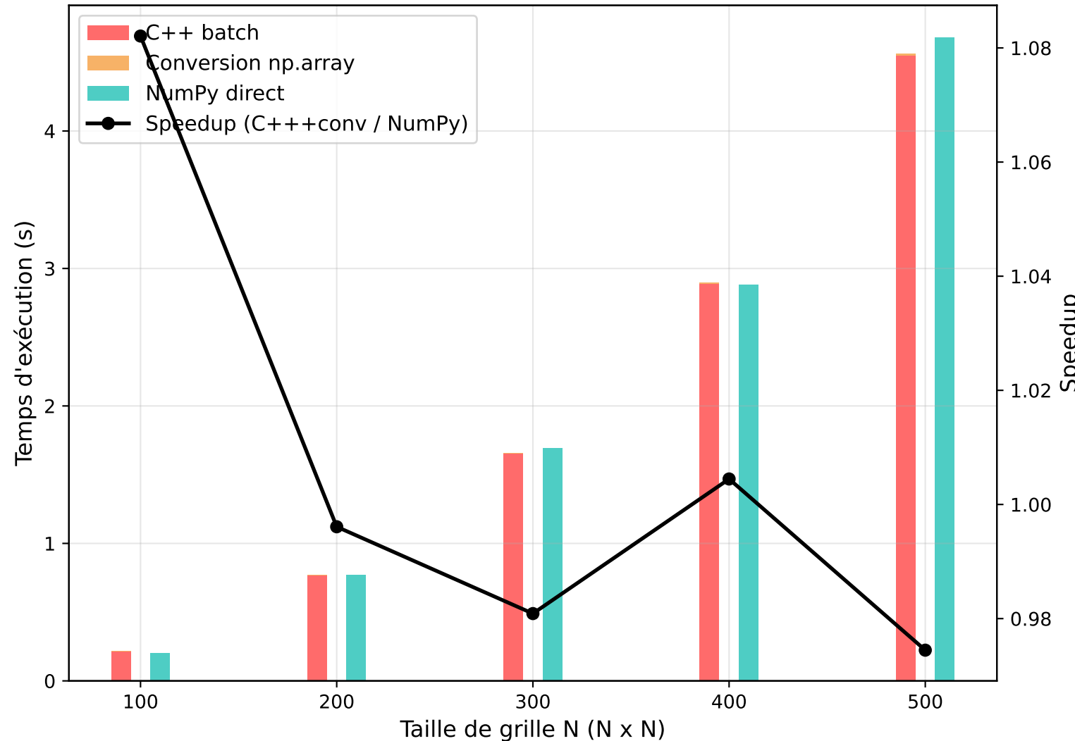
Benchmark C++ + conversion vs NumPy direct
