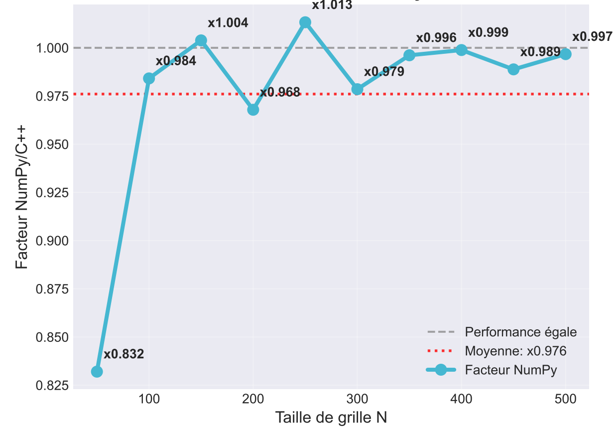
Performance relative NumPy vs C++
