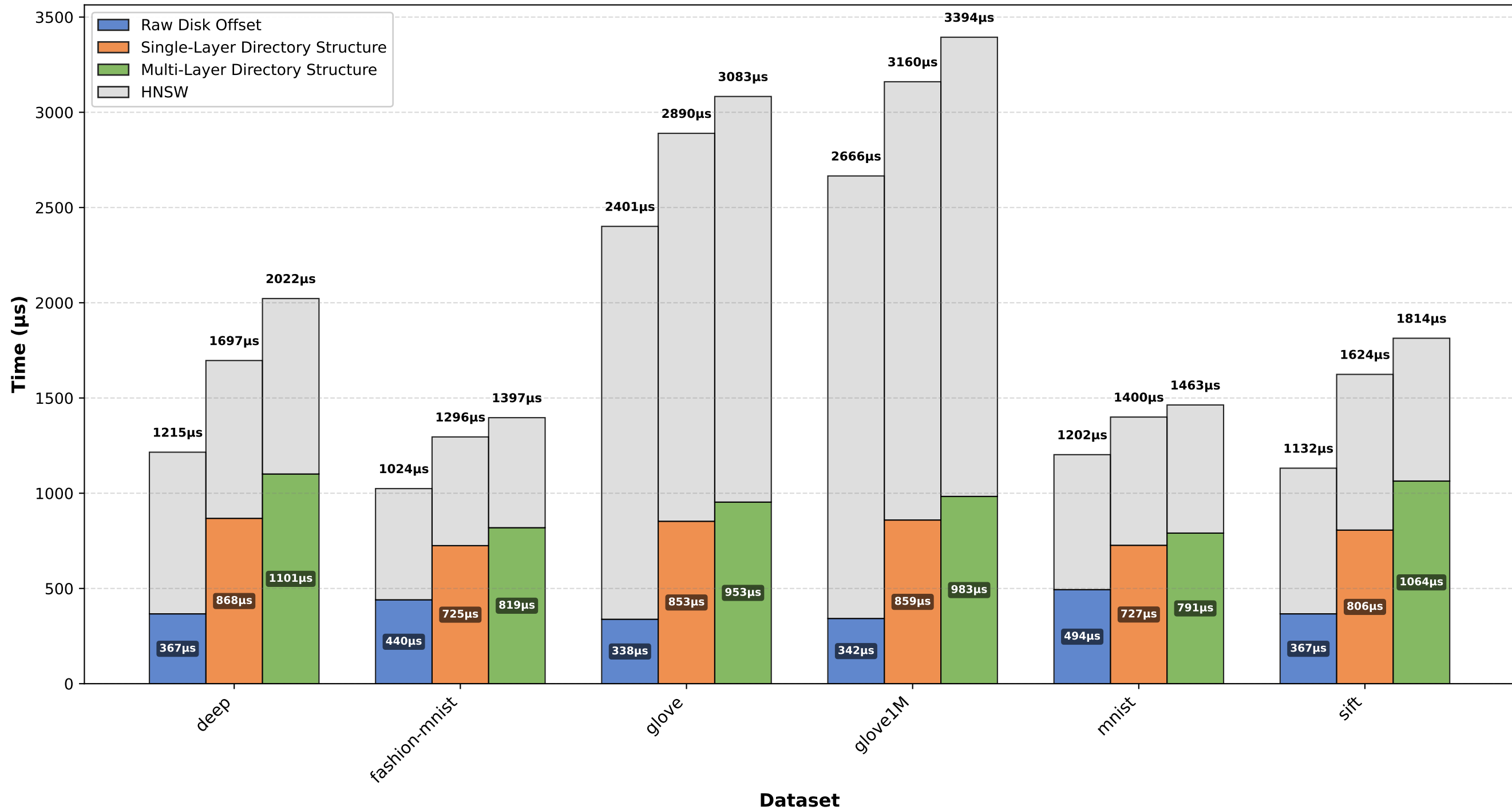
Query Latency Breakdown
