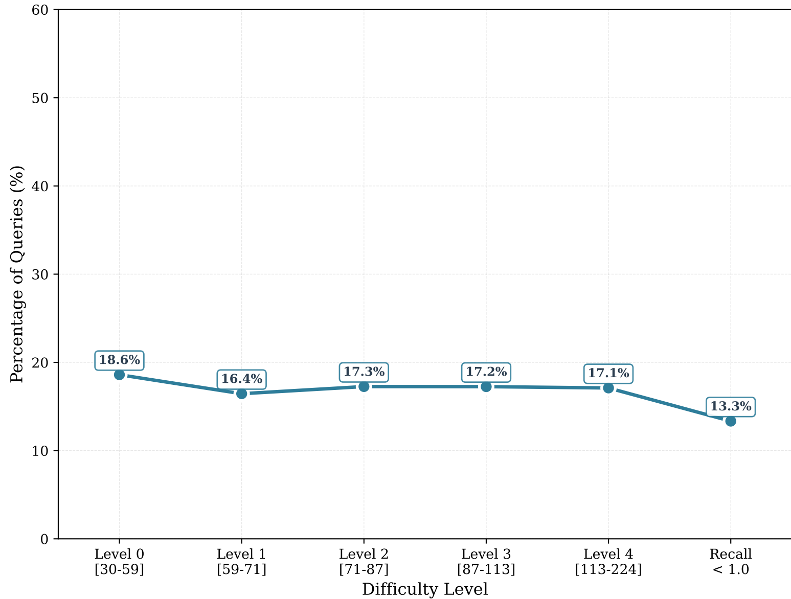
Fashion MNIST - Difficulty Distribution (EF=200)
