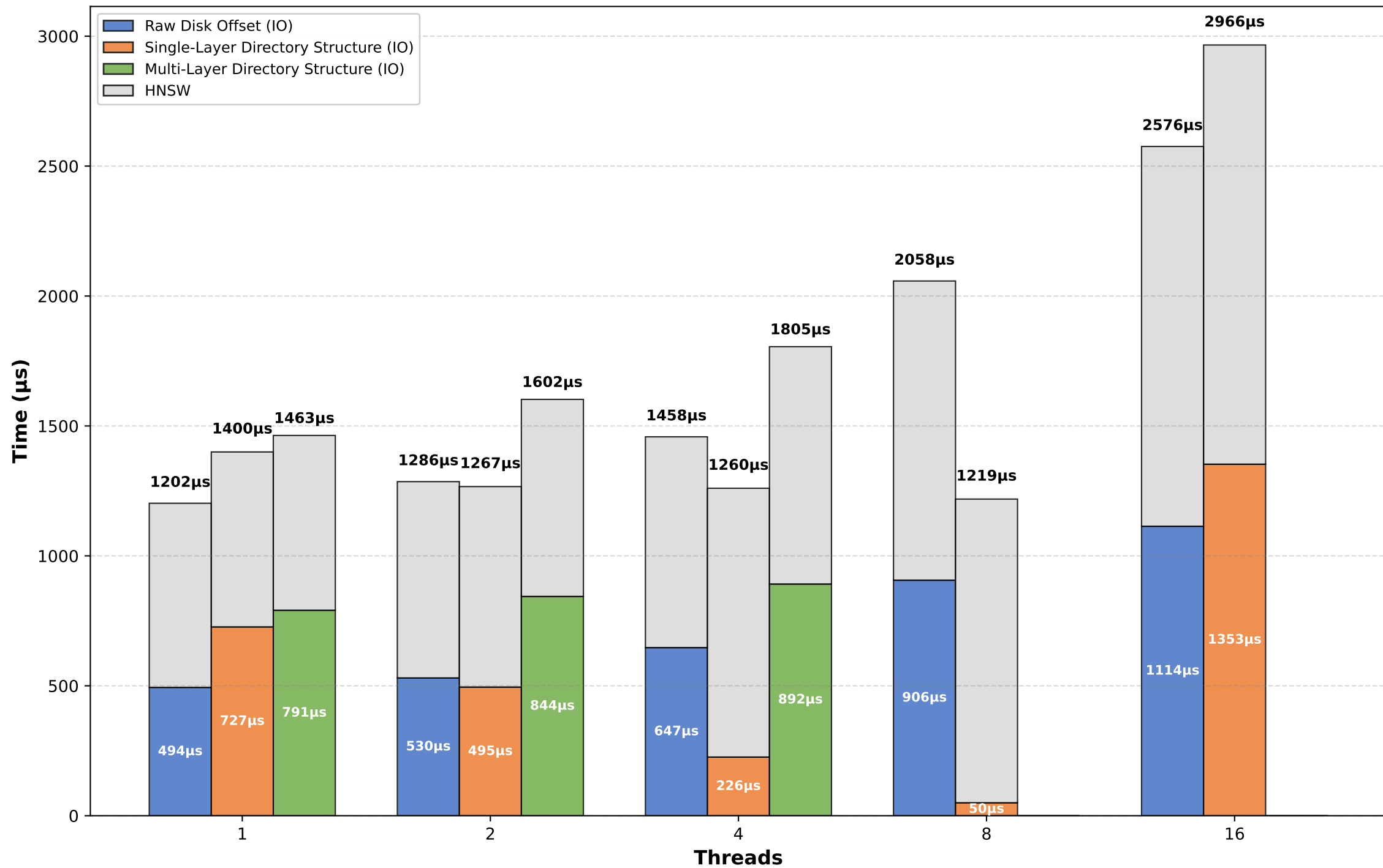
Latency Breakdown by Methods @ Dataset: mnist
