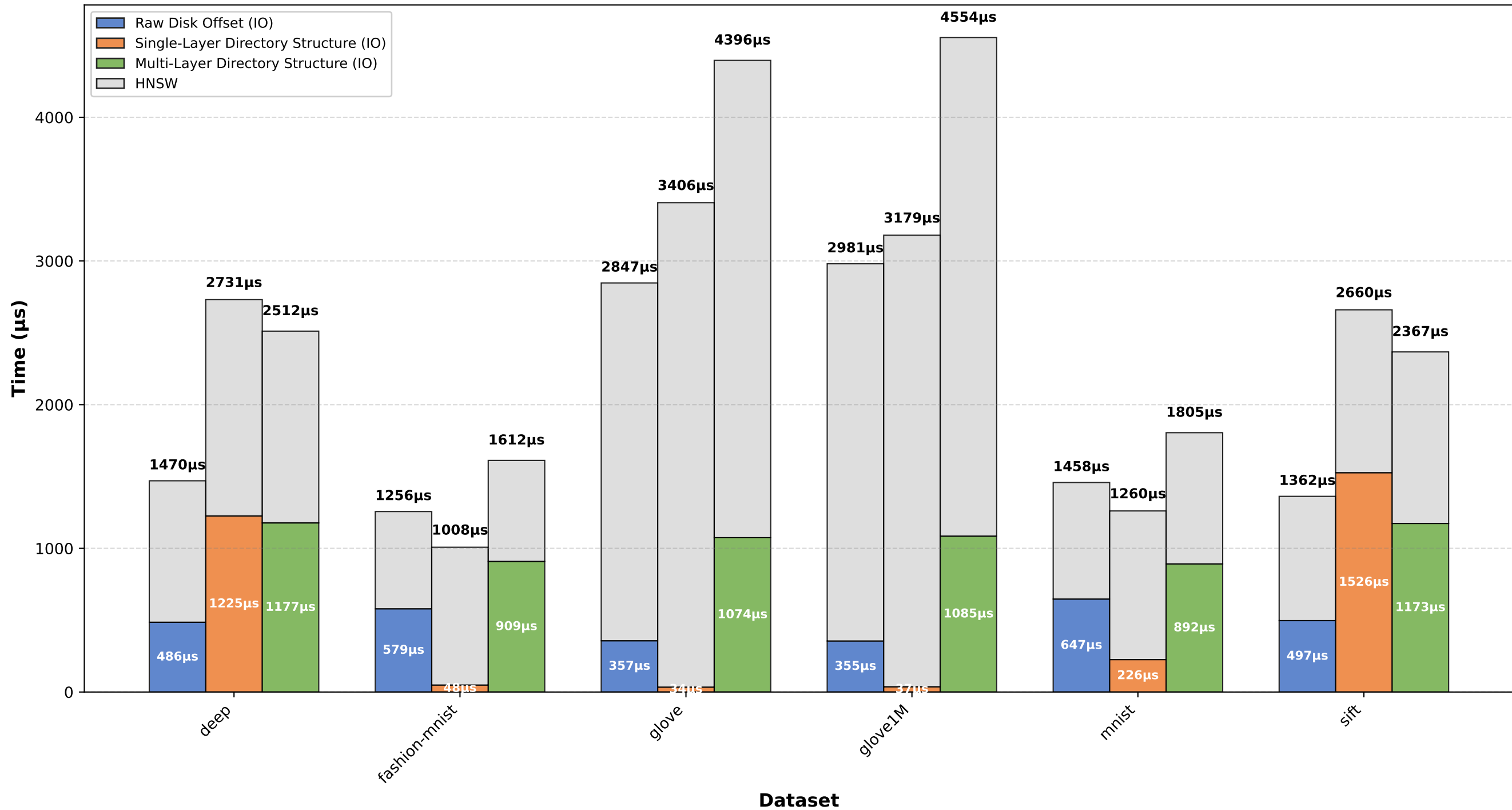
Latency Breakdown by Schemes @ 4 Threads
