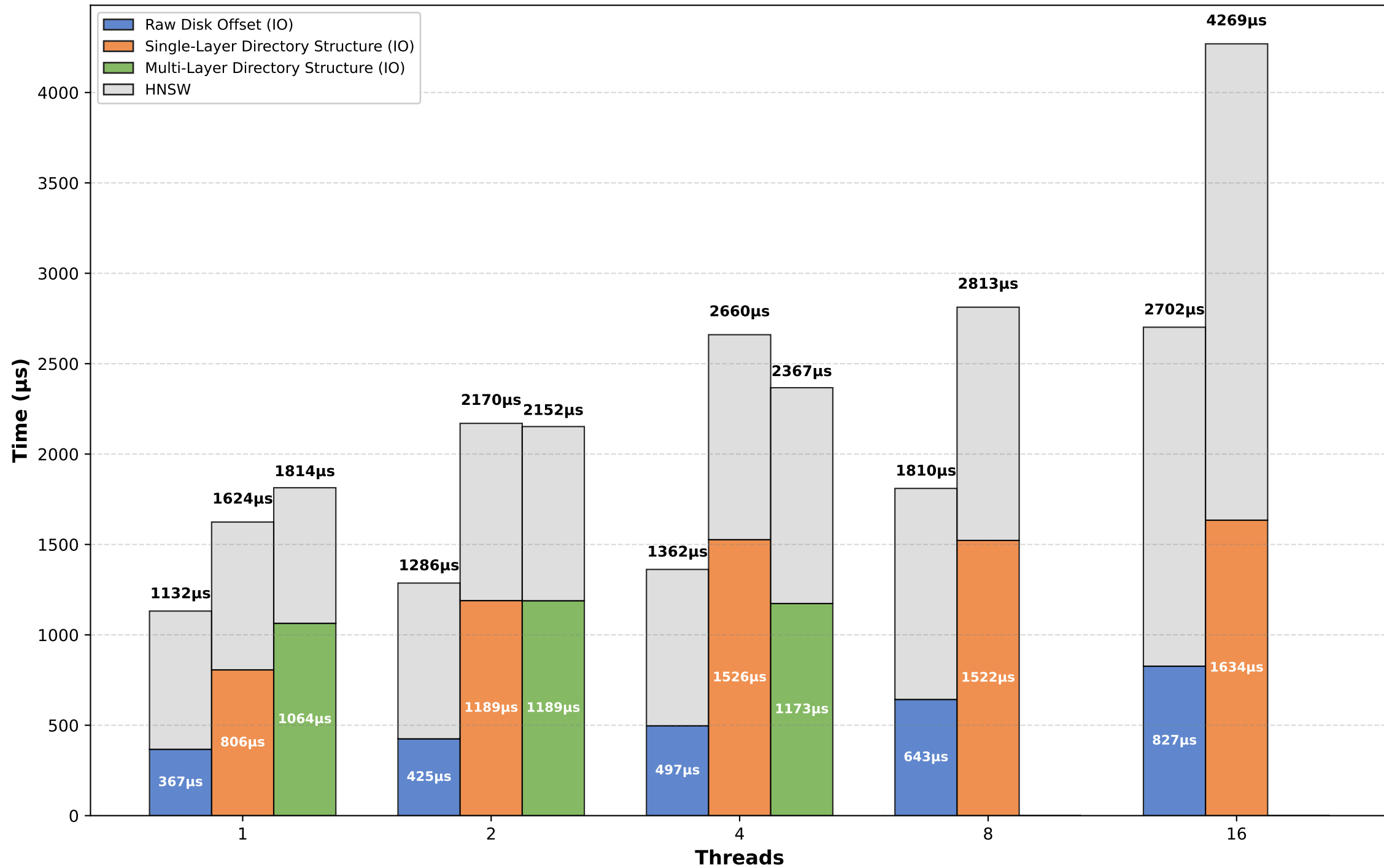
Latency Breakdown by Methods @ Dataset: sift
