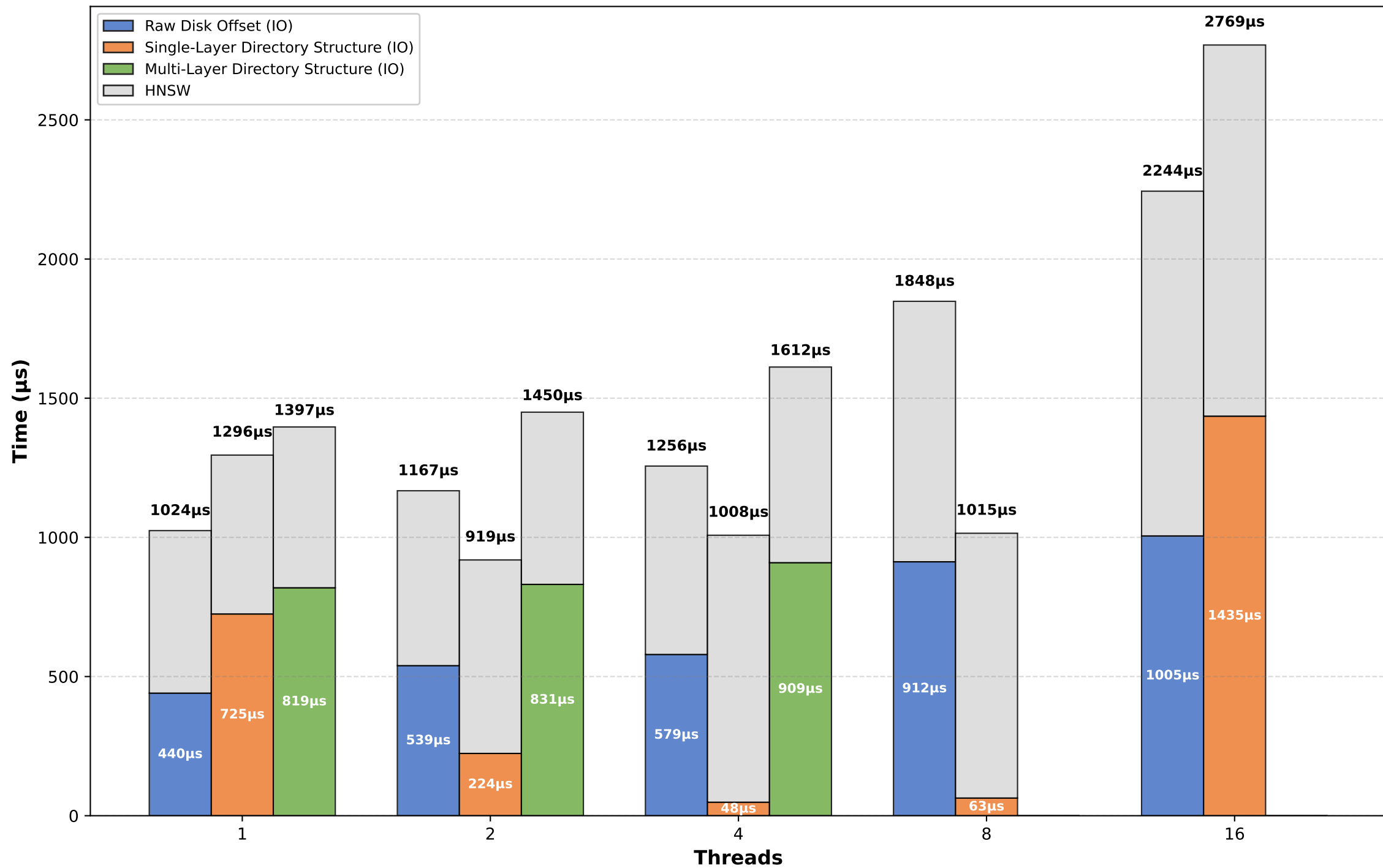
Latency Breakdown by Methods @ Dataset: fashion-mnist
