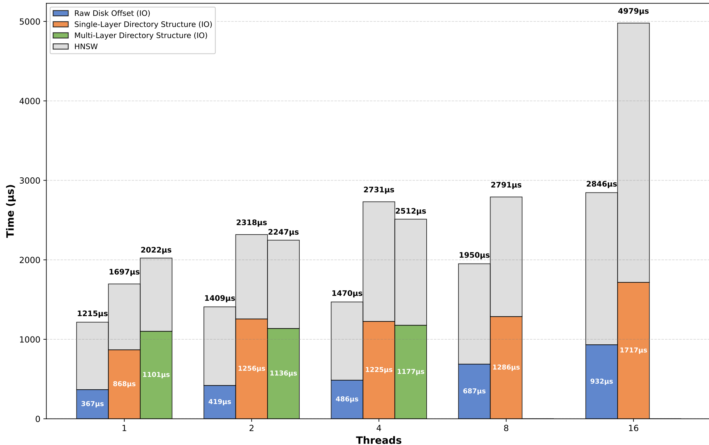
Latency Breakdown by Methods @ Dataset: deep
