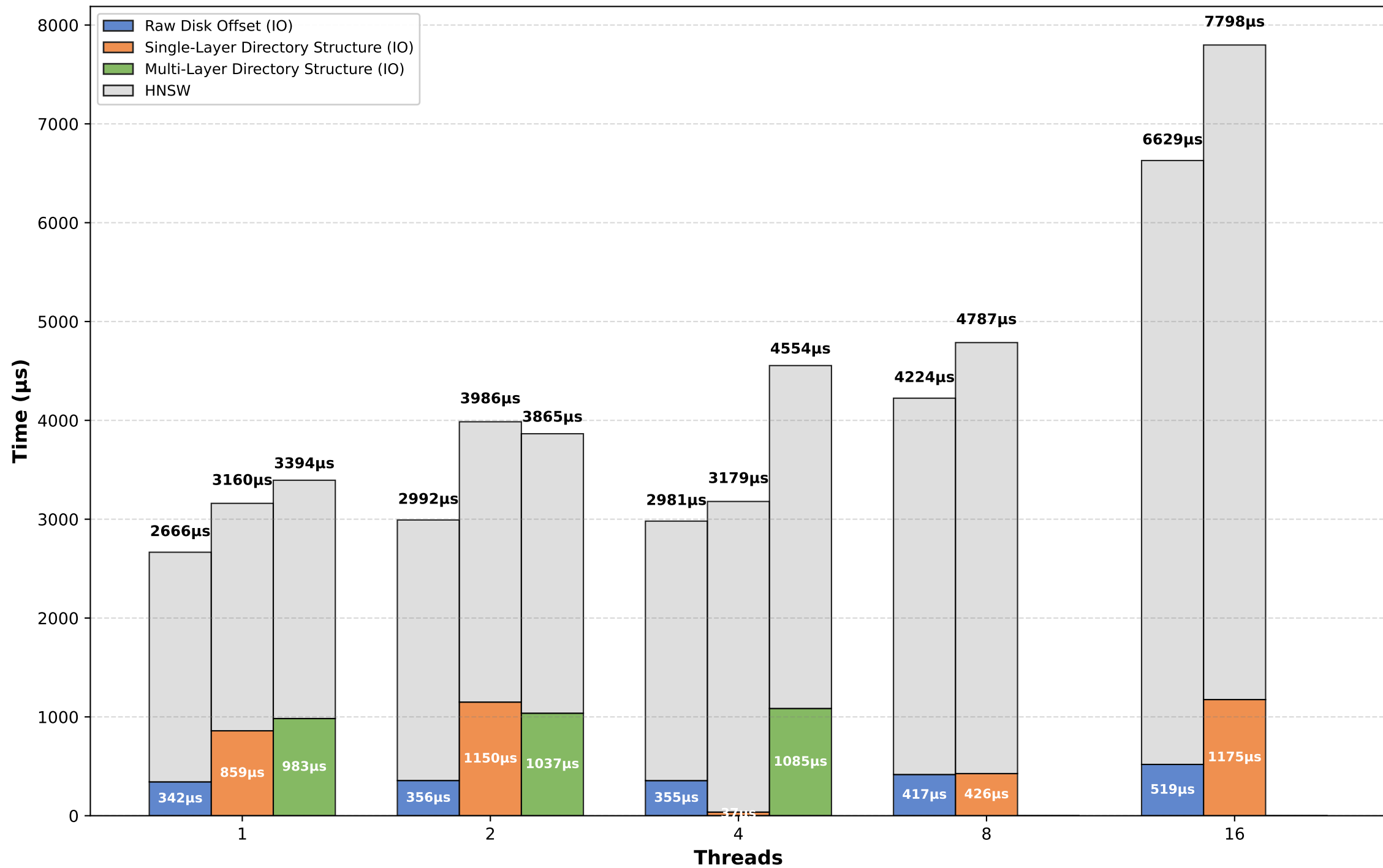
Latency Breakdown by Methods @ Dataset: glove1M
