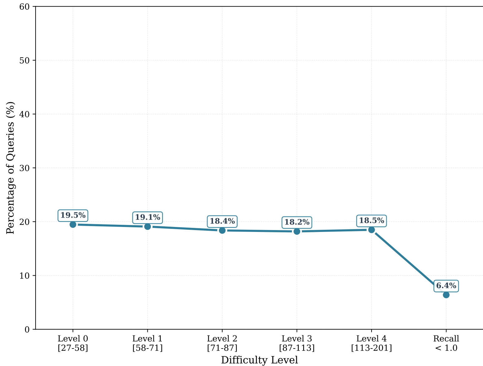
Mnist - Difficulty Distribution (EF=200)
