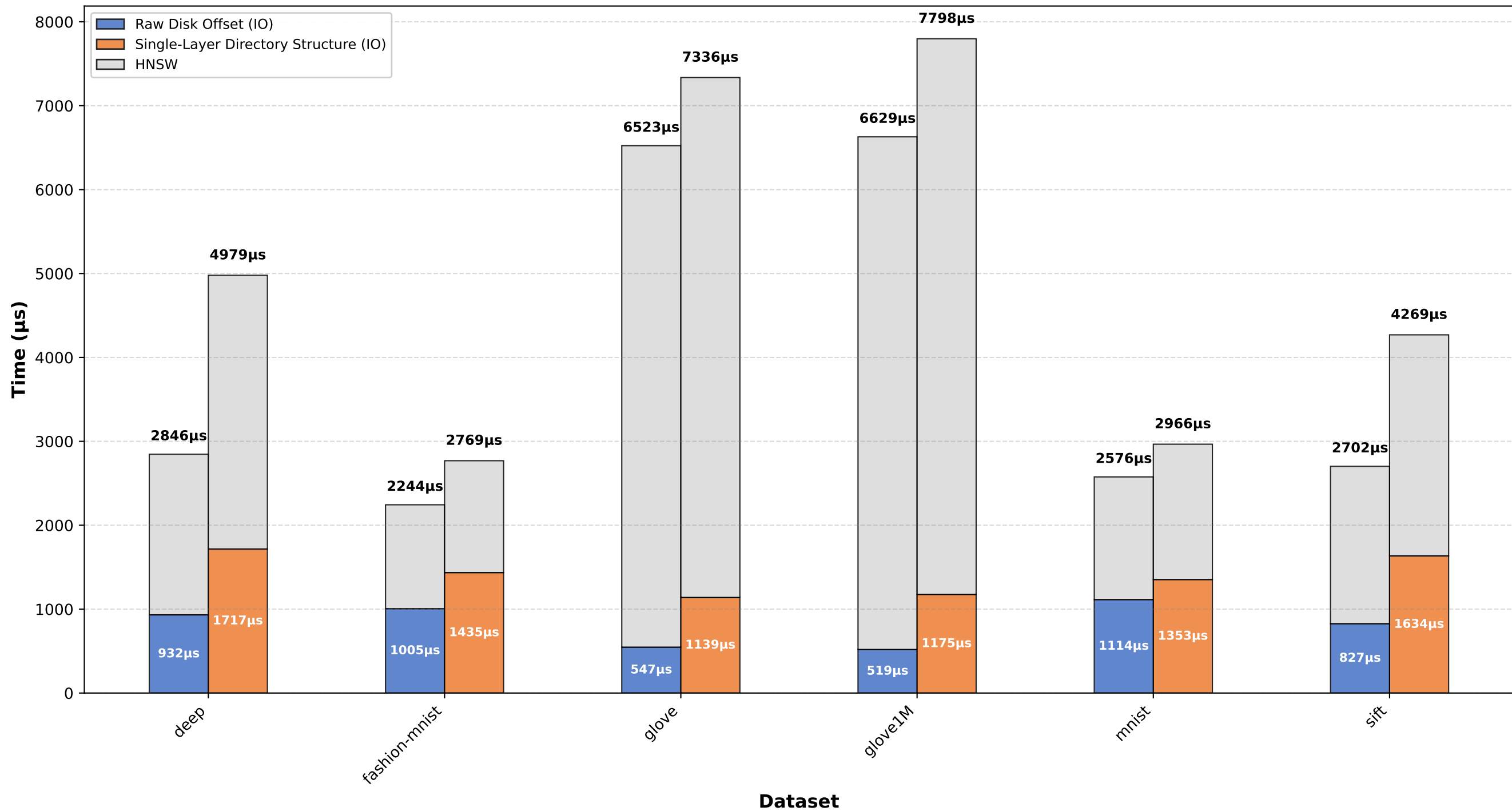
Latency Breakdown by Schemes @ 16 Threads
