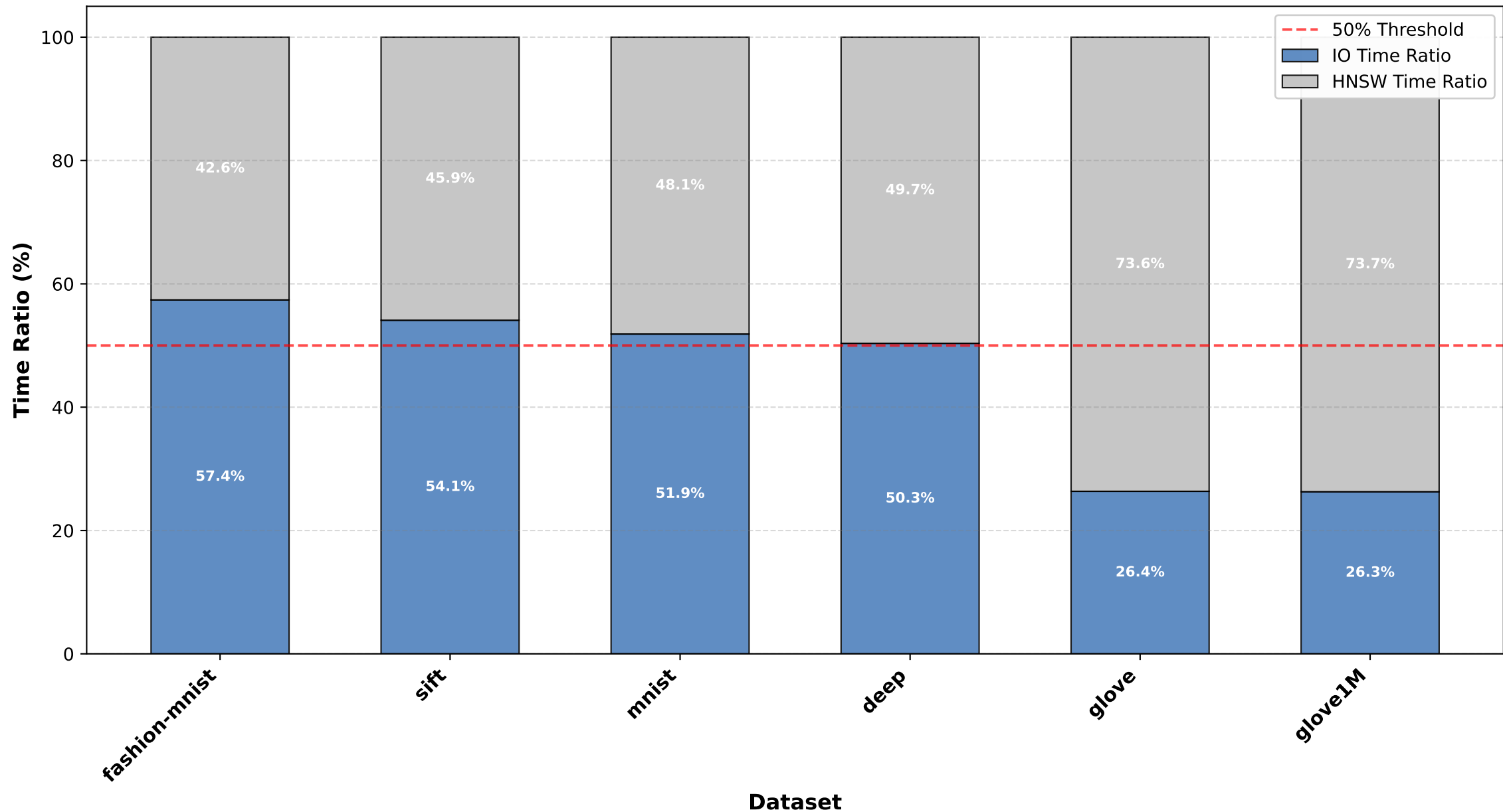
Multi-Level Directory: IO vs HNSW Time Ratio
