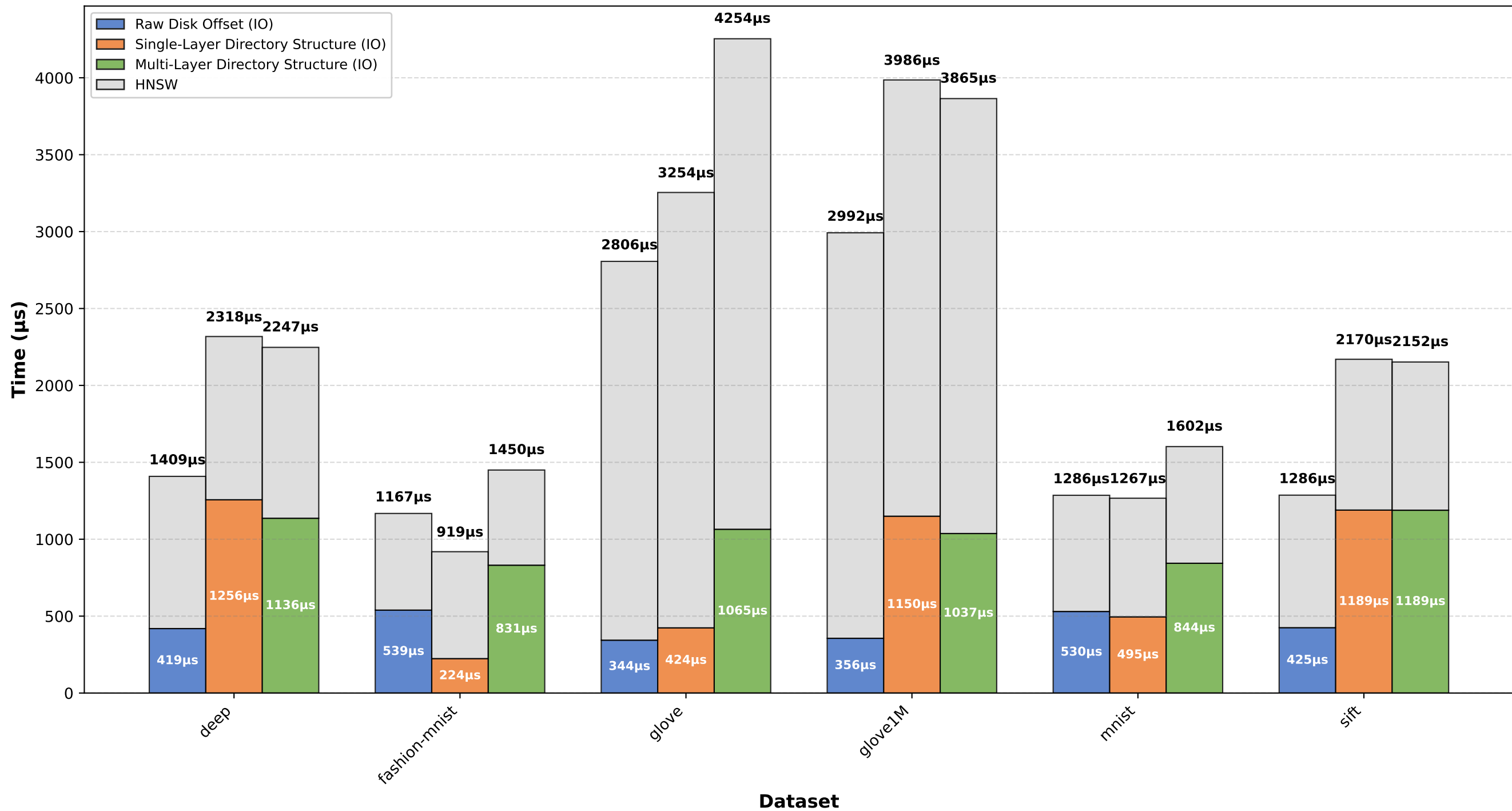
Latency Breakdown by Schemes @ 2 Threads
