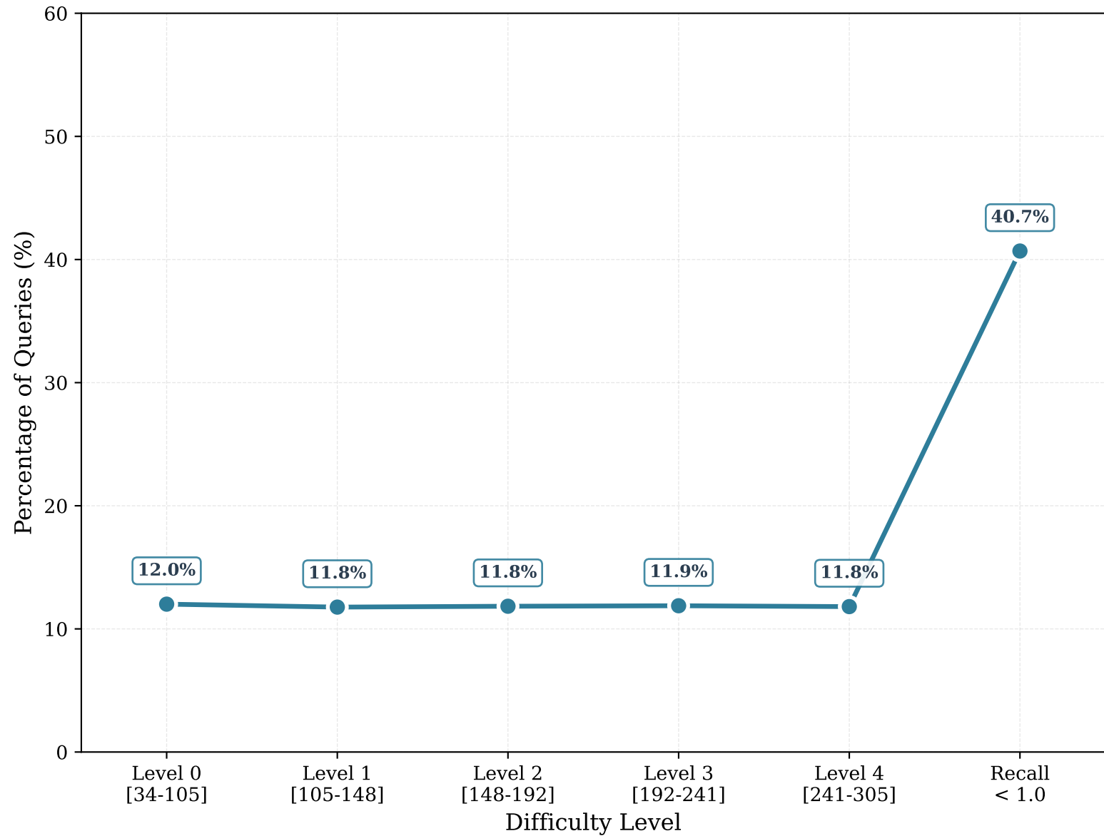
Sift - Difficulty Distribution (EF=300)
