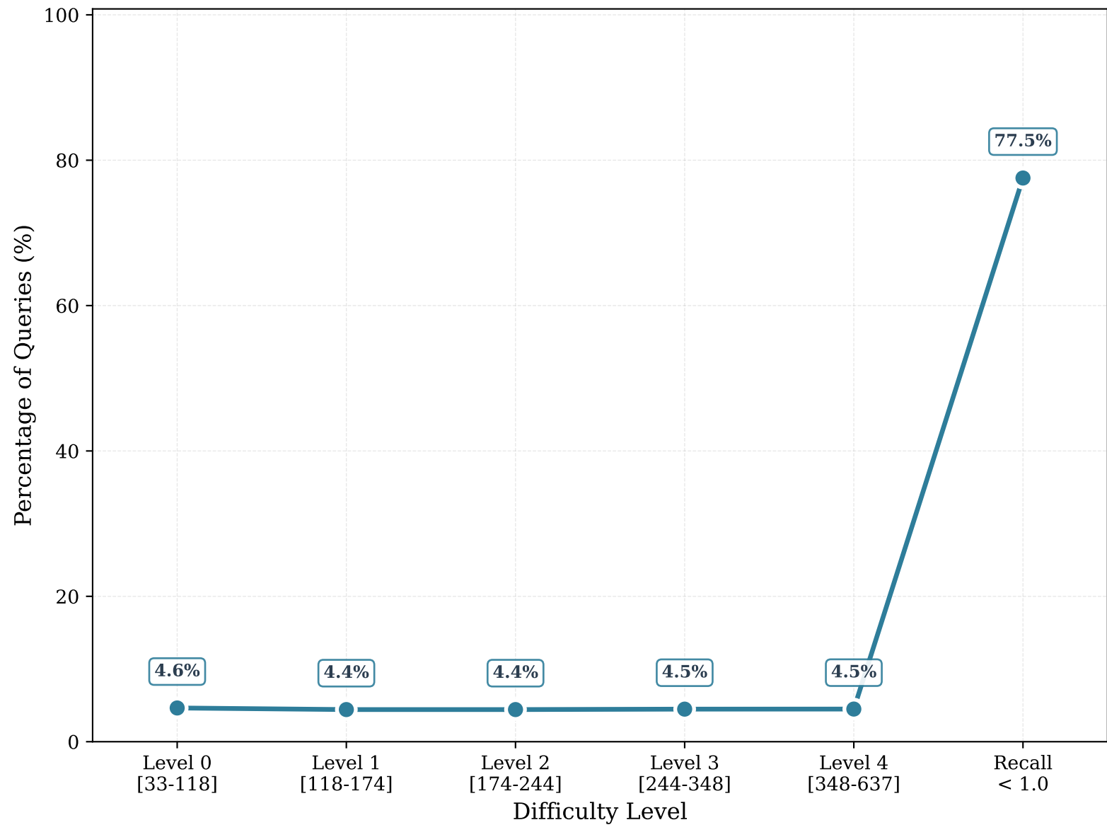
Glove - Difficulty Distribution (EF=500)
