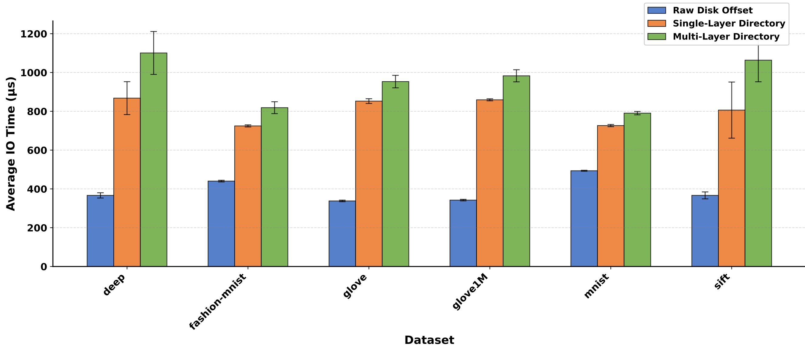
IO Latency Comparison Across Storage Schemes
