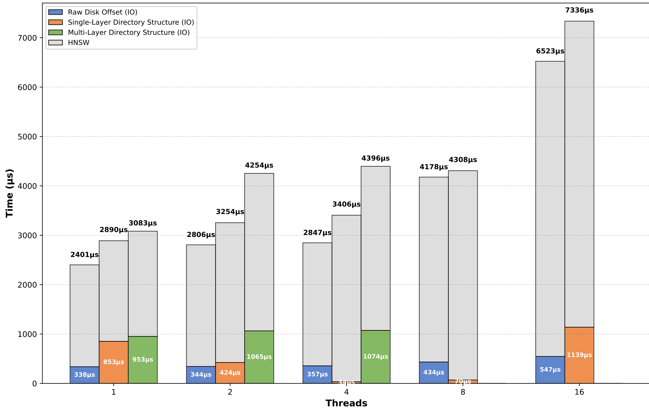
Latency Breakdown by Methods @ Dataset: glove
