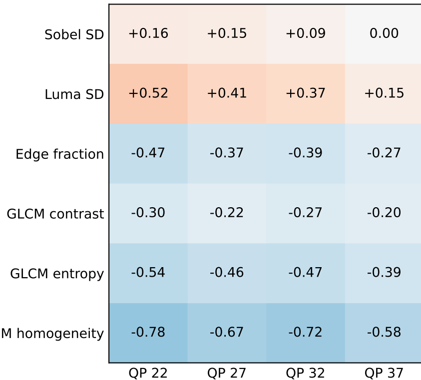
Kodak · 24 images Exploratory point estimates
