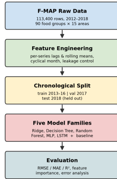
Fig. 1. End-to-end pipeline: data, feature engineering, chronological split, five model families, and evaluation.
