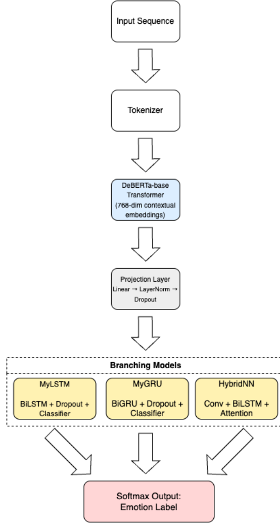
Figure 2: Pipeline: DeBERTa embeddings → projection → LSTM/GRU/CNN-LSTM → attention → classifier.
