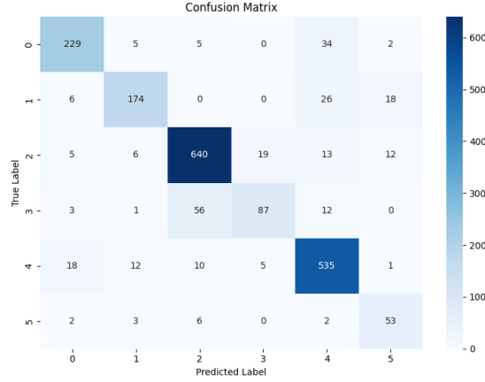
Figure 3: Confusion matrix
