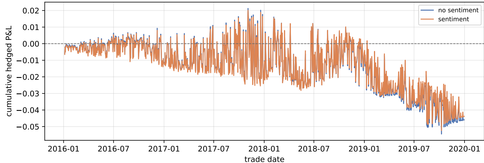
Delta-hedged P&L — Bates 2016-2019 variance NS 1.04e-04 | S 1.04e-04
