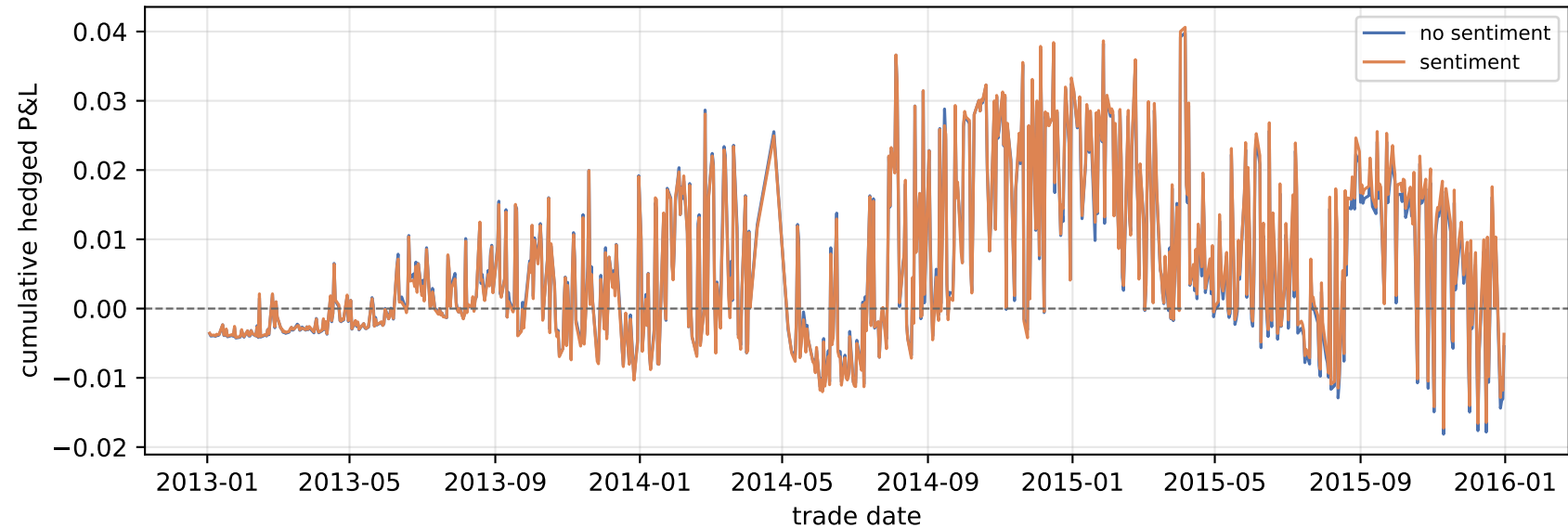
Delta-hedged P&L — Heston 2013-2015 variance NS 1.20\text{e-}04 | S 1.23\text{e-}04
